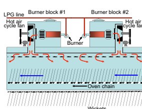
LACQUERING LINE OVEN
